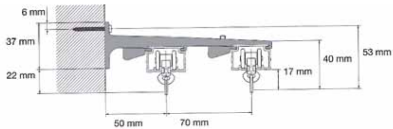
Support double Largeur support = 24 mm Suspendeur (00240011)
