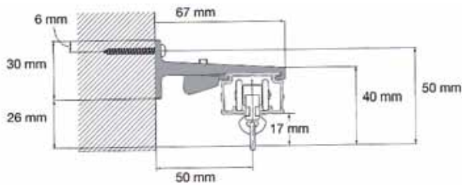
Support simple Largeur support = 20 mm Suspendeur (00240011)
